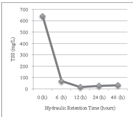
Fig. 3. TSS effluent in different HRT
