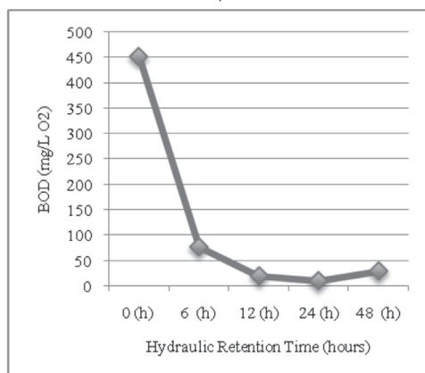
Fig. 5. BOD 5 effluent in different HRT
