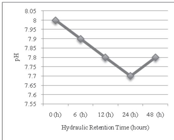
Fig. 2. pH effluent in different HRT
