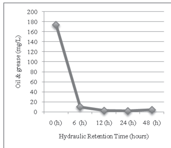
Fig. 6. Oil & grease effluent in different HRT
