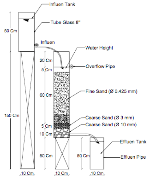
Fig. 1. Design of SSF prototype
