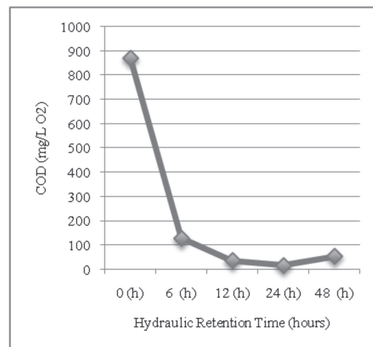
Fig. 4. COD effluent in different HRT
